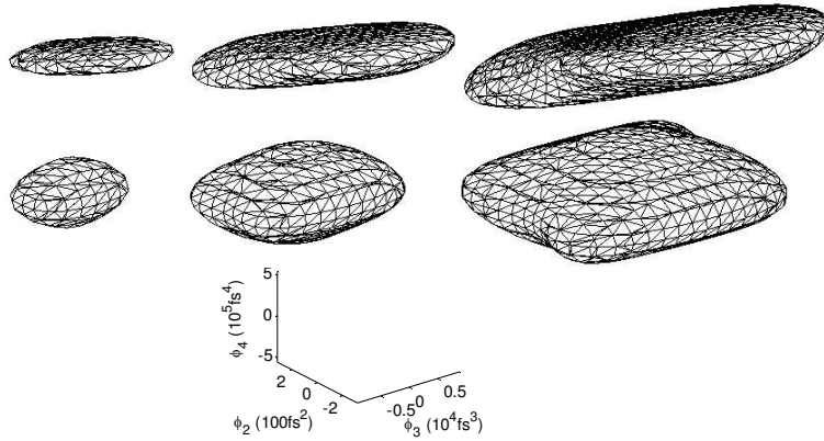
Fig. 6. The level sets of the 3D SHG landscape of the original (top) and modified (bottom) polynomials, corresponding to fitness values of 0.95 (left), 0.90 (middle), and 0.85 (right). All 3D level sets are viewed in the same Cartesian coordinate and from the same angle (azimuth = -37.5^\circ , elevation = 30^\circ ). See the attached animated GIF for the evolution of the level sets.
